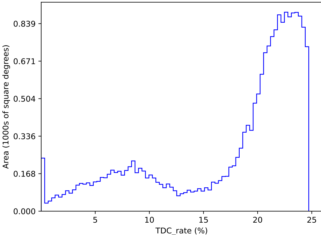
internal_u_expt38_nscale1.5v3.4_10yrs : TDC_rate
