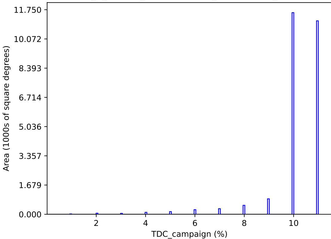
internal_u_expt38_nscale1.5v3.4_10yrs : TDC_campaign
