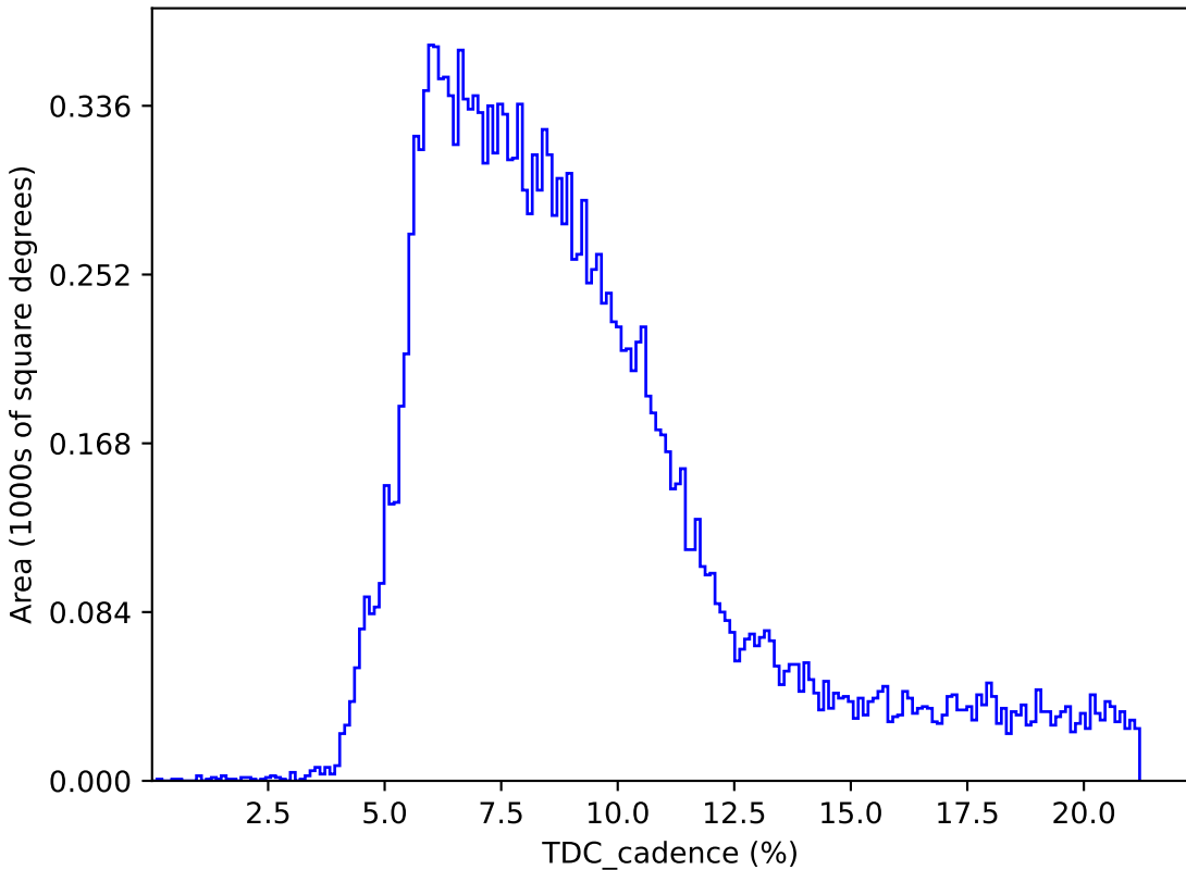
internal_u_expt38_nscale1.5v3.4_10yrs : TDC_cadence
