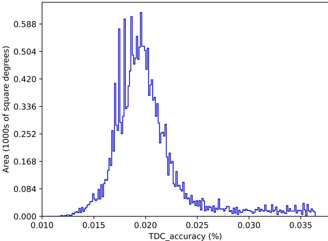
internal_u_expt38_nscale1.5v3.4_10yrs : TDC_accuracy
