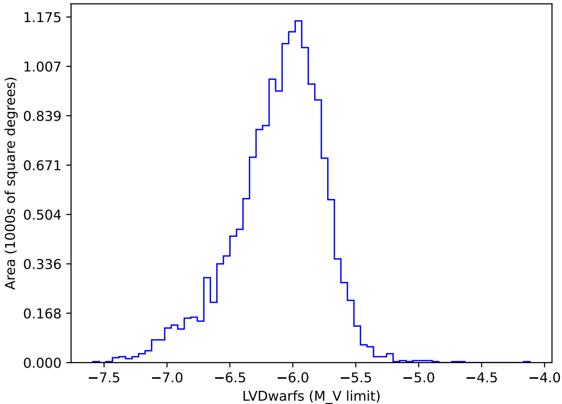
internal_u_expt38_nscale1.5v3.4_10yrs gi: LVDwarfs
