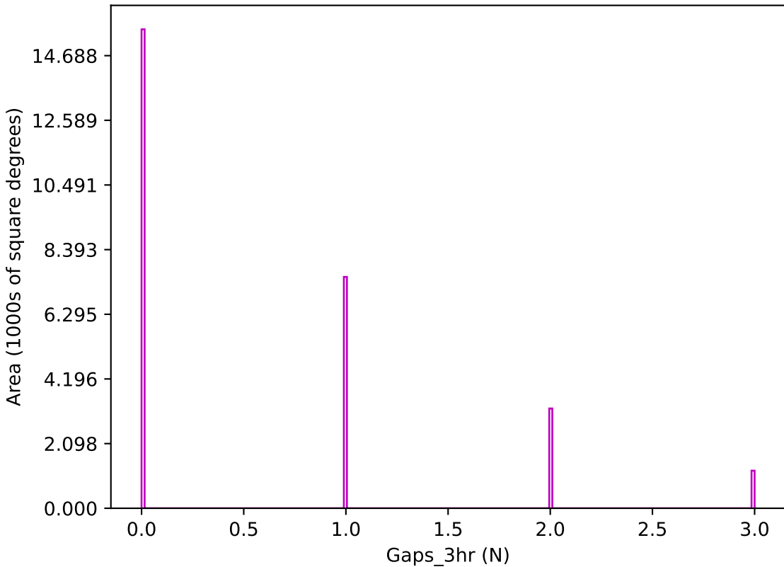
internal_u_expt38_nscale1.5v3.4_10yrs z band: Gaps_3hr
