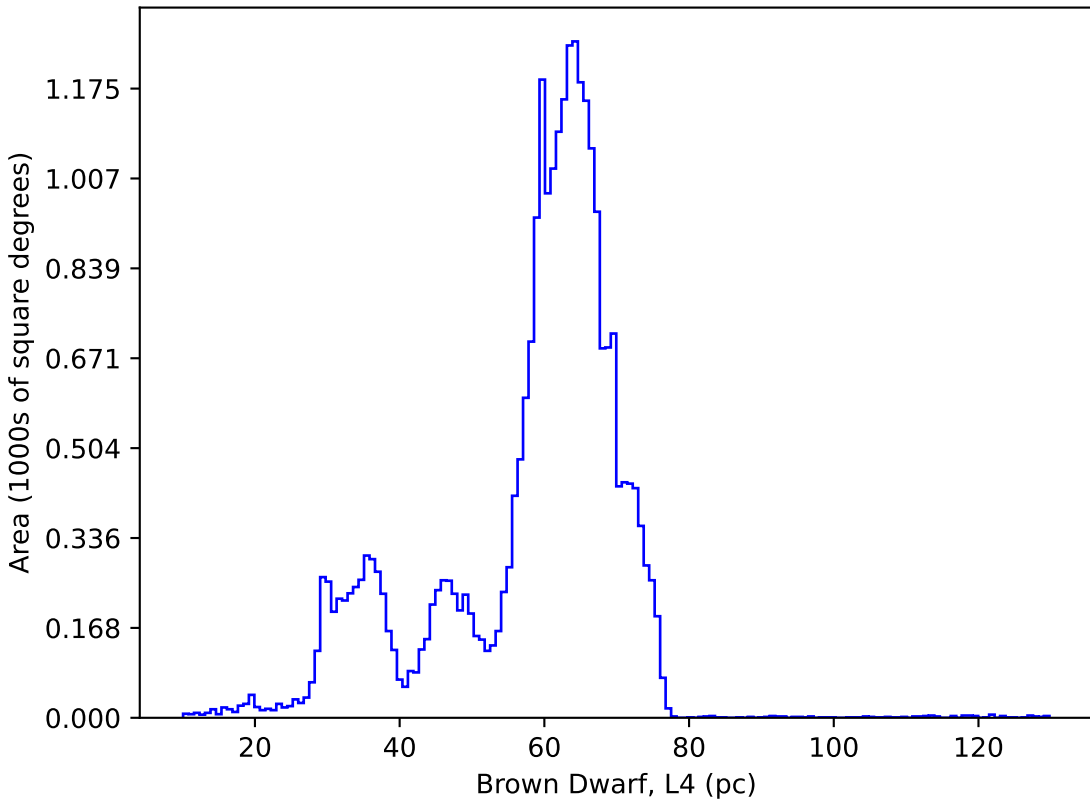
internal_u_expt38_nscale1.5v3.4_10yrs : Brown Dwarf, L4
