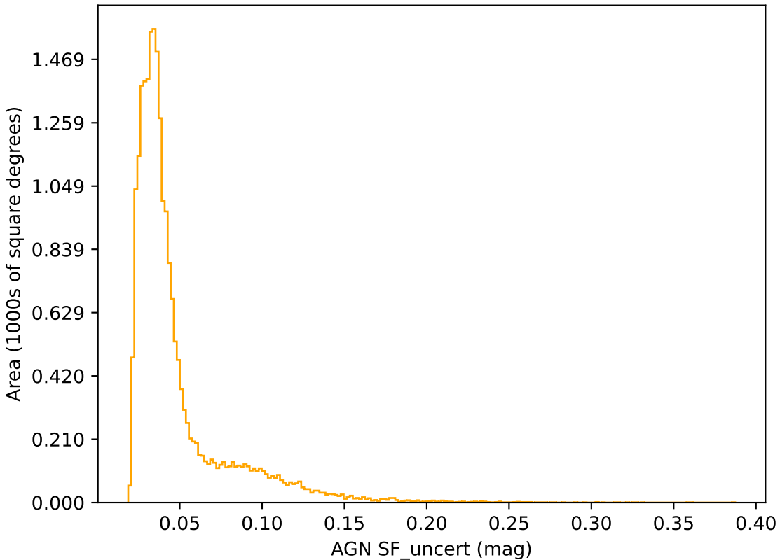
internal_u_expt38_nscale1.5v3.4_10yrs r band: AGN SF_uncert
