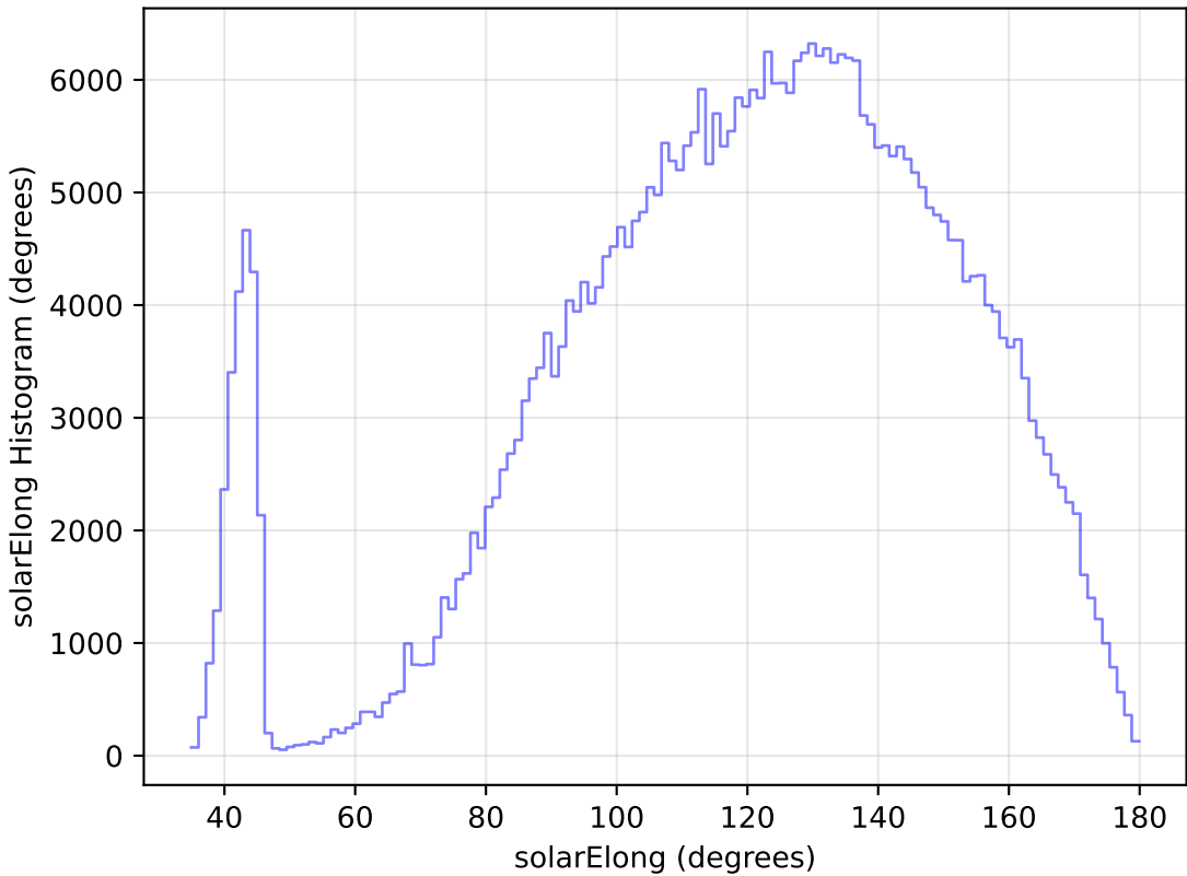
internal_u_expt38_nscale1.5v3.4_10yrs WFD z band: solarElong Histogram
