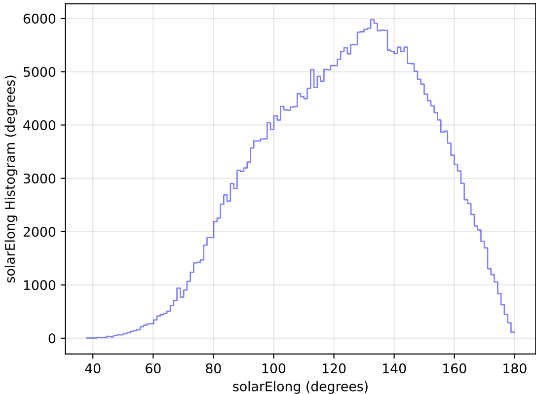
internal_u_expt38_nscale1.5v3.4_10yrs WFD y band: solarElong Histogram
