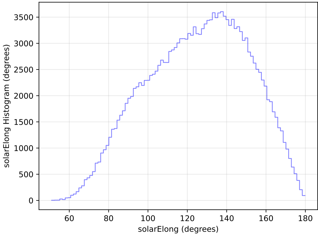
internal_u_expt38_nscale1.5v3.4_10yrs WFD u band: solarElong Histogram
