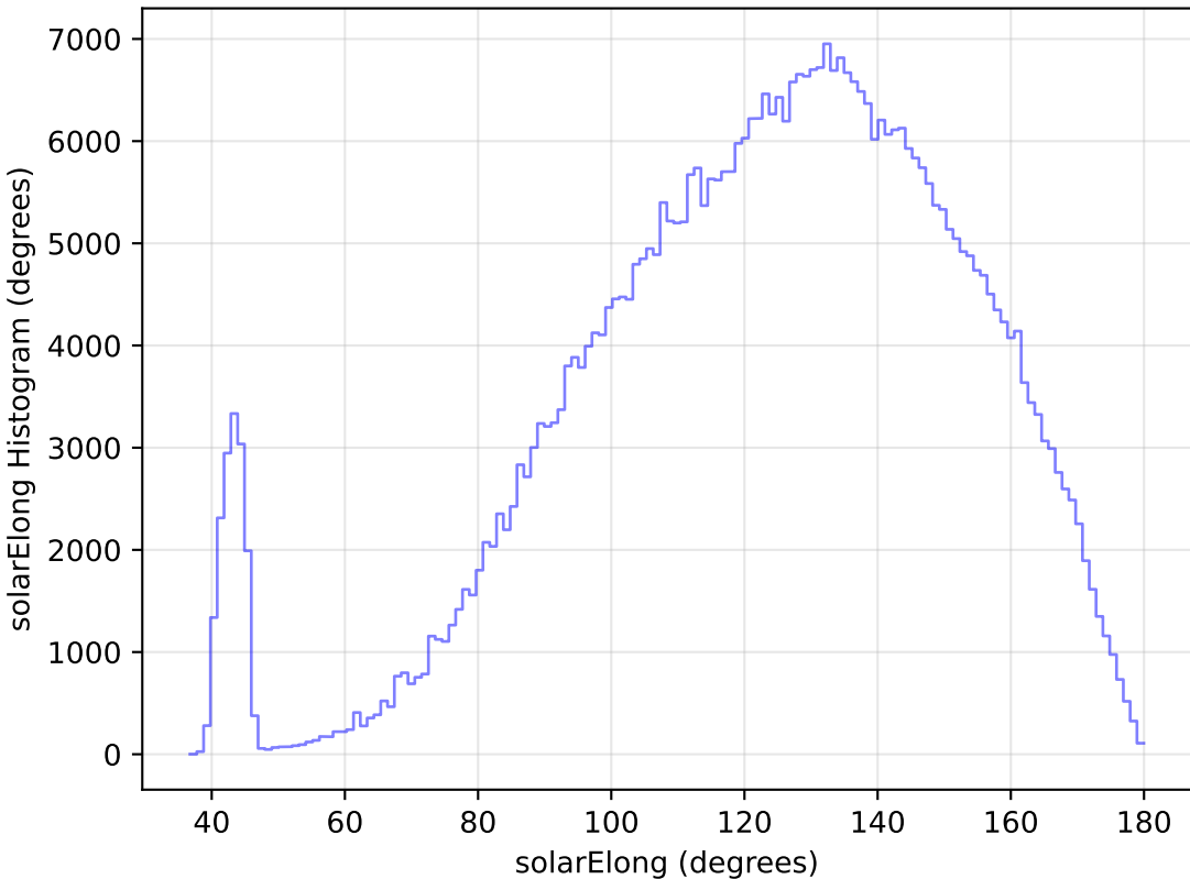
internal_u_expt38_nscale1.5v3.4_10yrs WFD r band: solarElong Histogram
