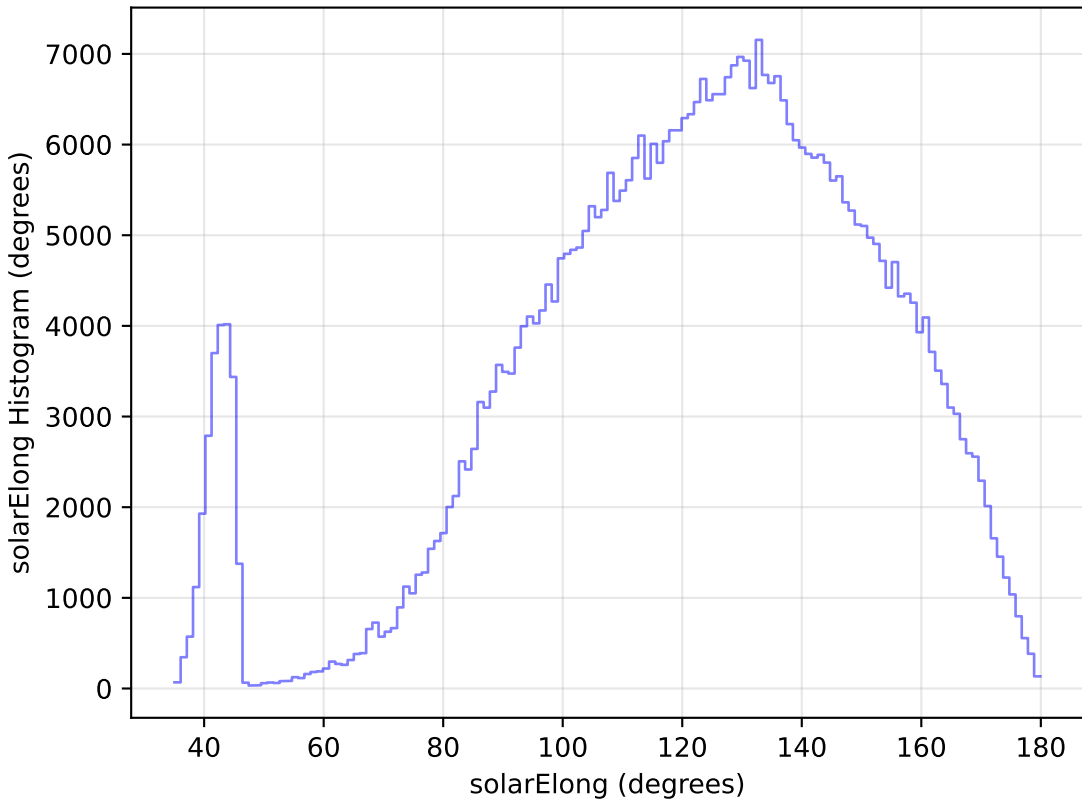
internal_u_expt38_nscale1.5v3.4_10yrs WFD i band: solarElong Histogram
