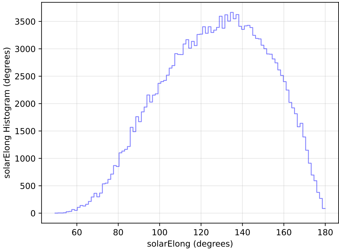
internal_u_expt38_nscale1.5v3.4_10yrs WFD g band: solarElong Histogram
