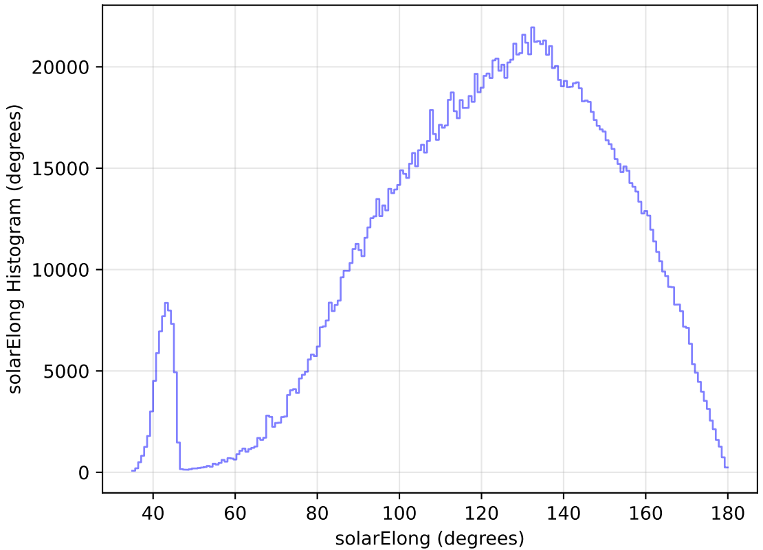
internal_u_expt38_nscale1.5v3.4_10yrs WFD all bands: solarElong Histogram
