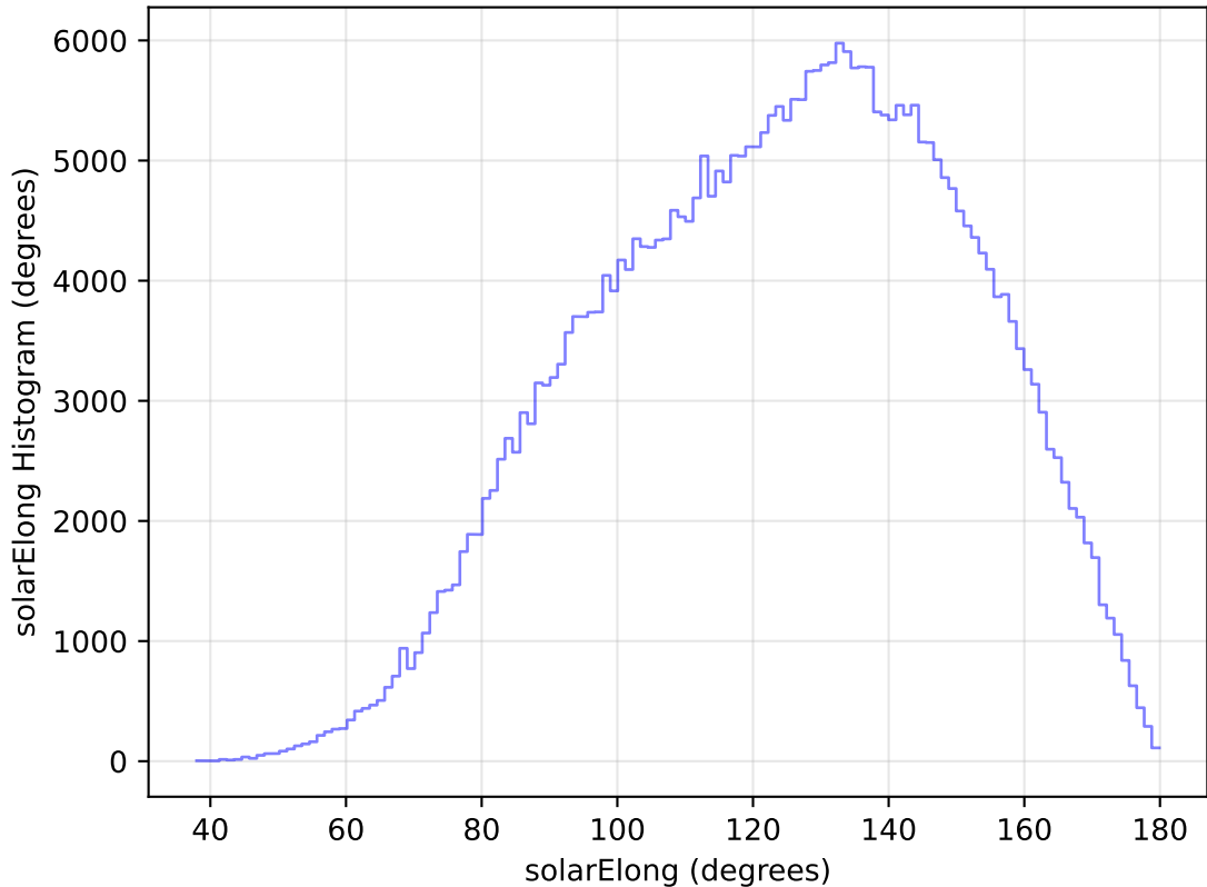
internal_u_expt38_nscale1.5v3.4_10yrs All sky y band: solarElong Histogram
