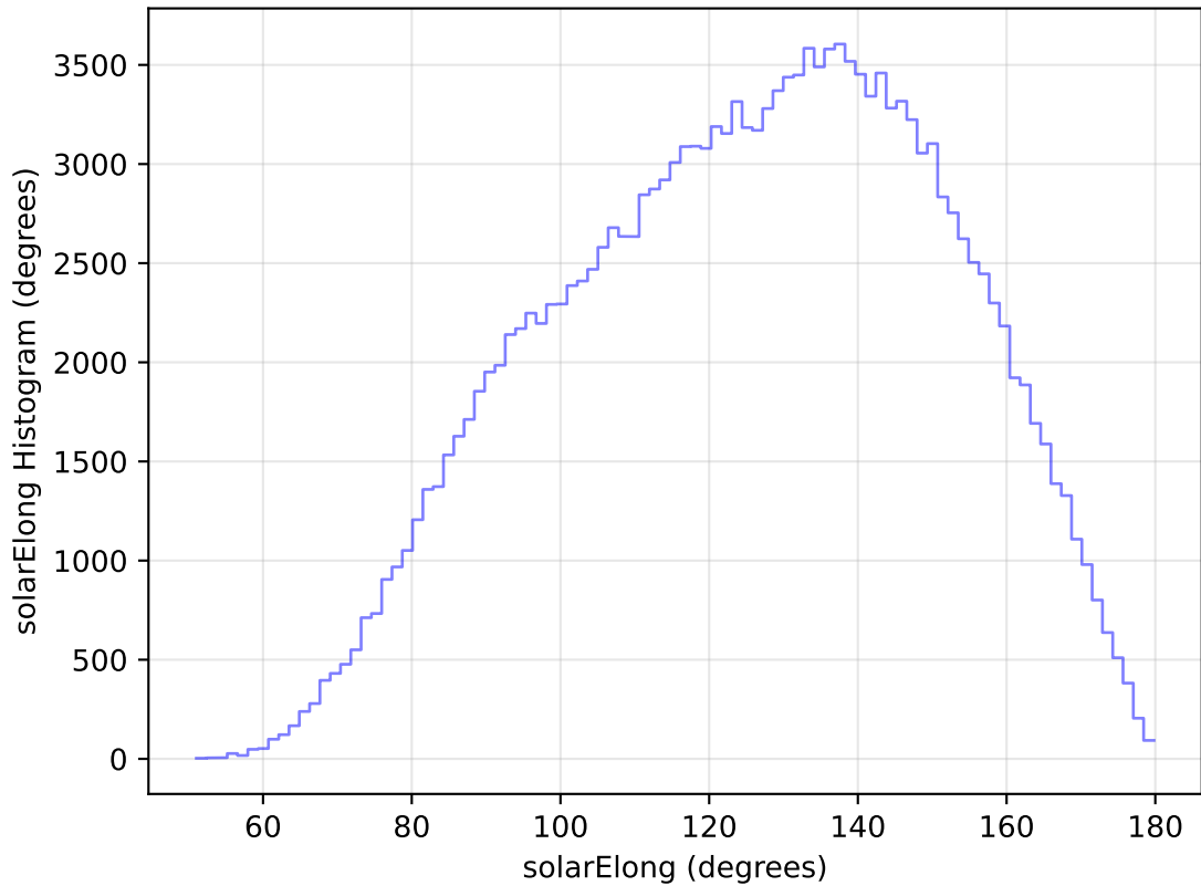
internal_u_expt38_nscale1.5v3.4_10yrs All sky u band: solarElong Histogram
