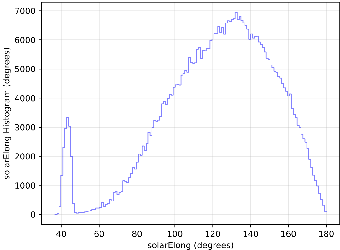
internal_u_expt38_nscale1.5v3.4_10yrs All sky r band: solarElong Histogram
