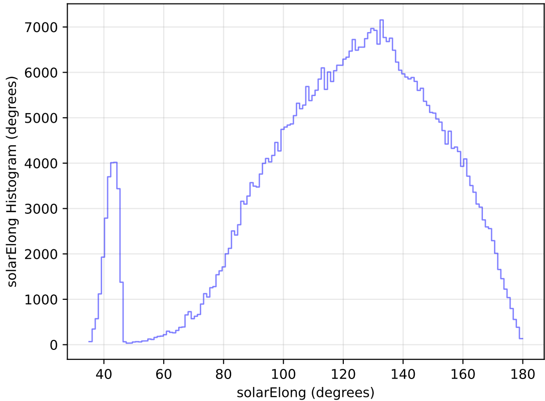
internal_u_expt38_nscale1.5v3.4_10yrs All sky i band: solarElong Histogram
