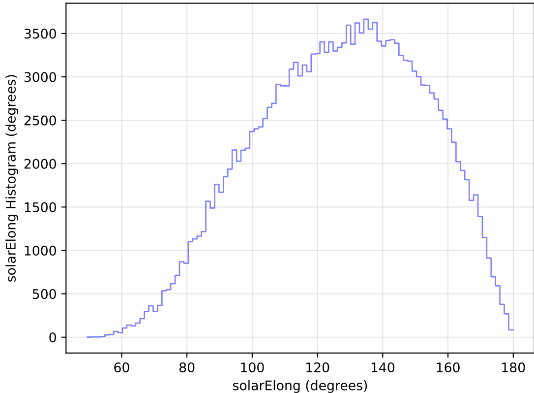
internal_u_expt38_nscale1.5v3.4_10yrs All sky g band: solarElong Histogram
