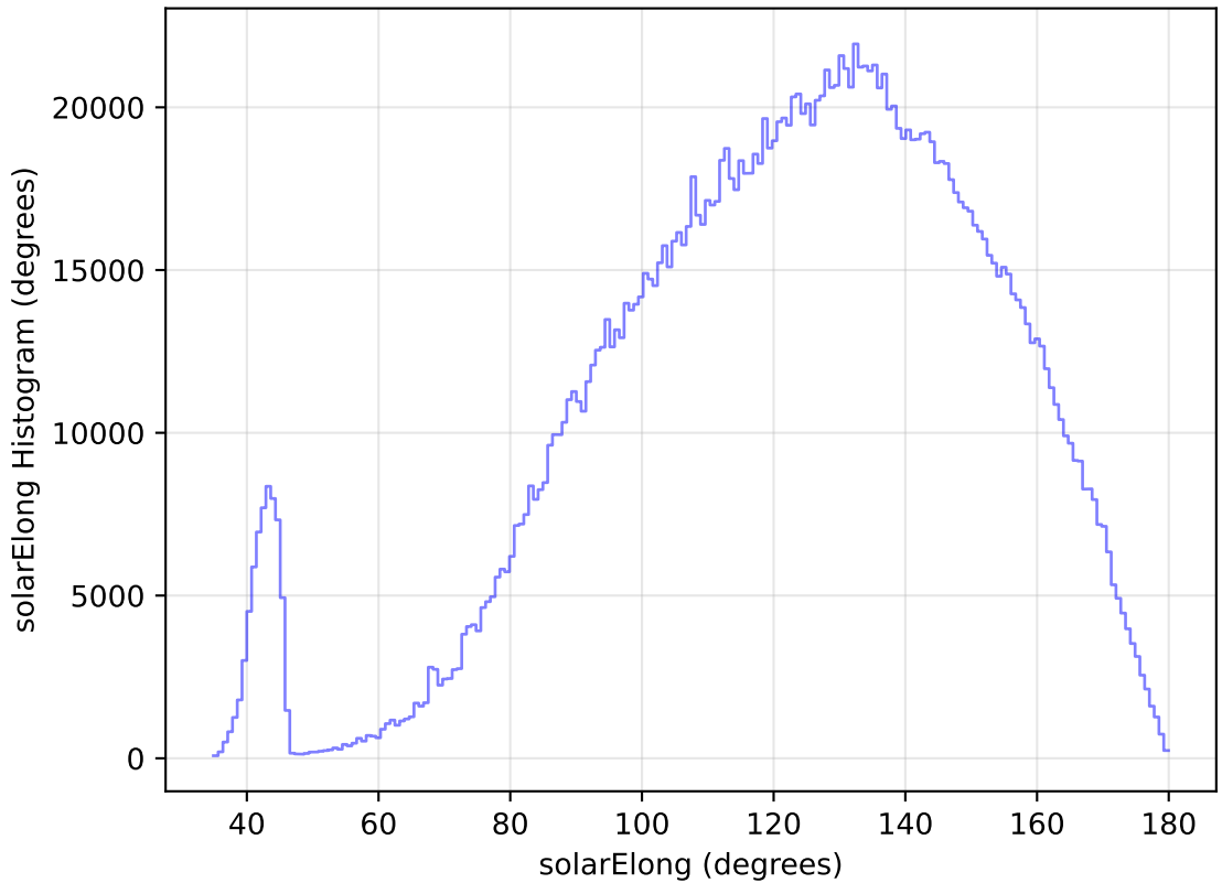
internal_u_expt38_nscale1.5v3.4_10yrs All sky all bands: solarElong Histogram
