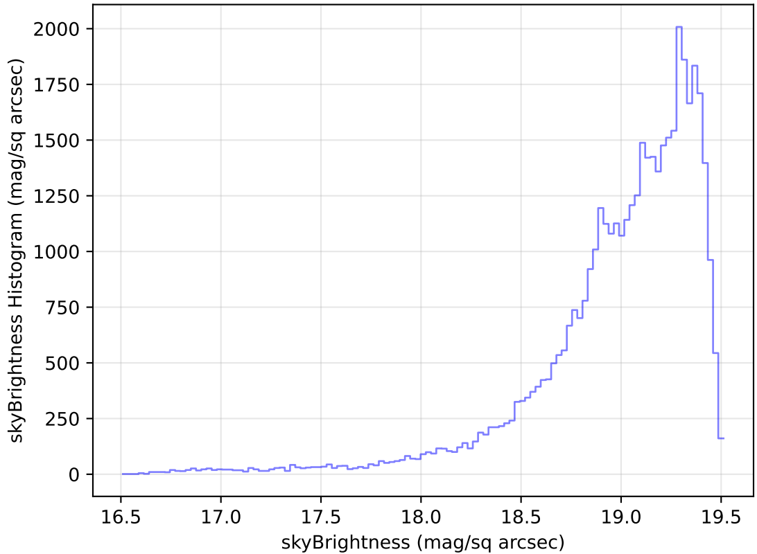
internal_u_expt38_nscale1.5v3.4_10yrs Yr 1 z band: skyBrightness Histogram
