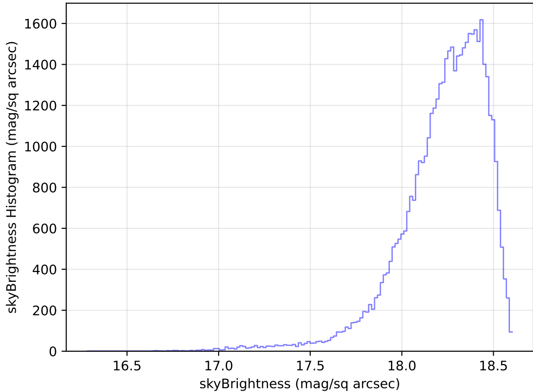
internal_u_expt38_nscale1.5v3.4_10yrs Yr 1 y band: skyBrightness Histogram
