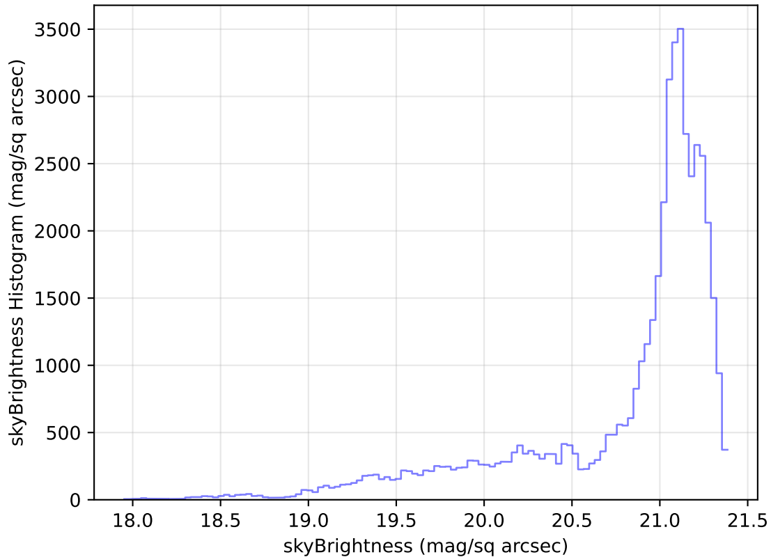
internal_u_expt38_nscale1.5v3.4_10yrs Yr 1 r band: skyBrightness Histogram
