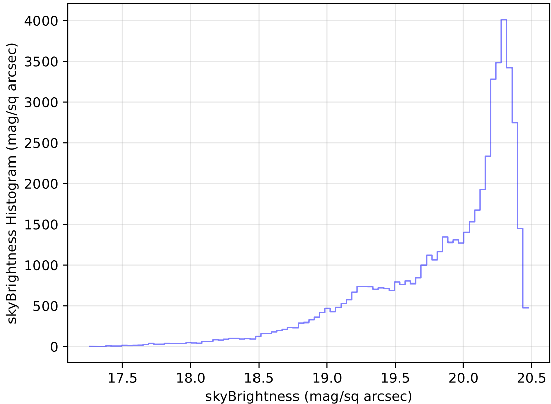
internal_u_expt38_nscale1.5v3.4_10yrs Yr 1 i band: skyBrightness Histogram
