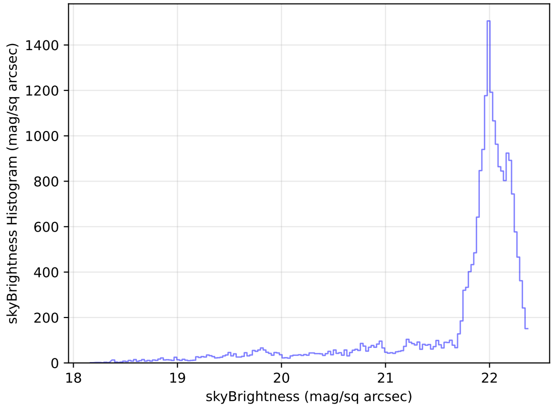
internal_u_expt38_nscale1.5v3.4_10yrs Yr 1 g band: skyBrightness Histogram
