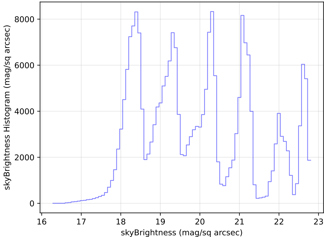
internal_u_expt38_nscale1.5v3.4_10yrs Yr 1 all bands: skyBrightness Histogram
