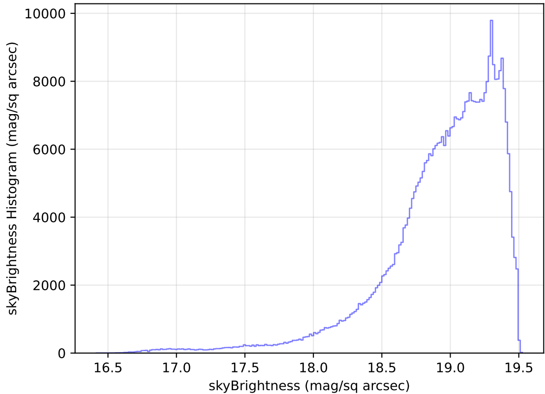
internal_u_expt38_nscale1.5v3.4_10yrs WFD z band: skyBrightness Histogram
