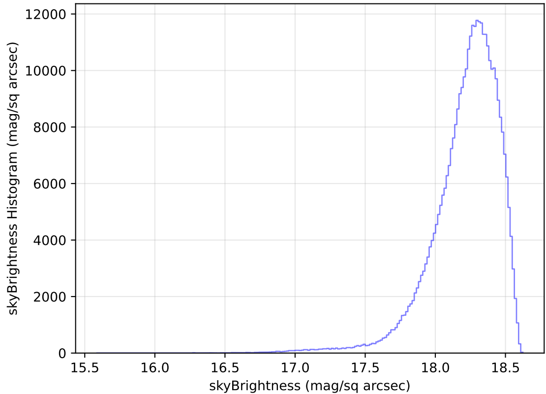
internal_u_expt38_nscale1.5v3.4_10yrs WFD y band: skyBrightness Histogram
