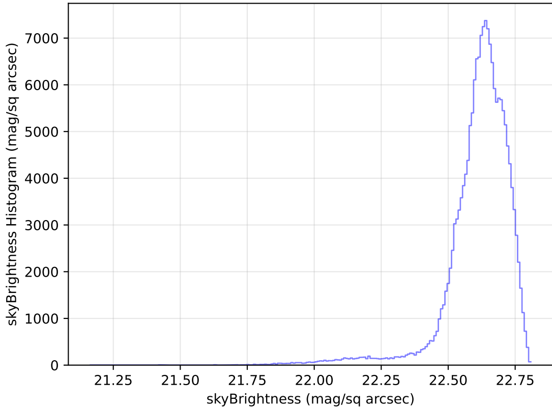
internal_u_expt38_nscale1.5v3.4_10yrs WFD u band: skyBrightness Histogram
