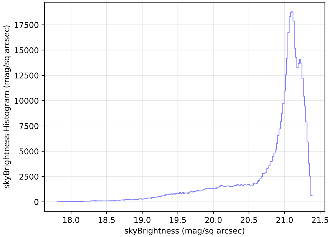
internal_u_expt38_nscale1.5v3.4_10yrs WFD r band: skyBrightness Histogram
