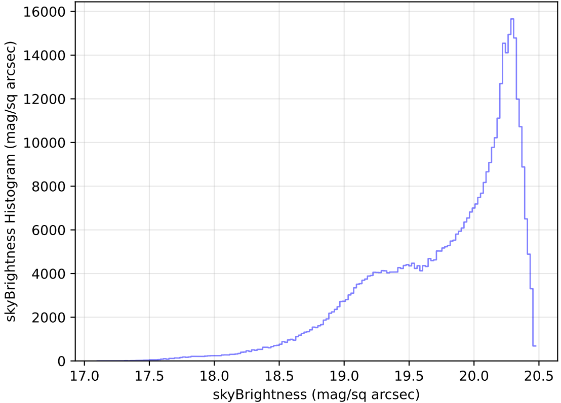
internal_u_expt38_nscale1.5v3.4_10yrs WFD i band: skyBrightness Histogram
