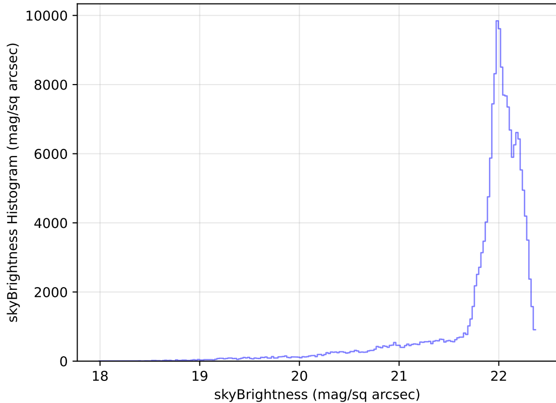
internal_u_expt38_nscale1.5v3.4_10yrs WFD g band: skyBrightness Histogram
