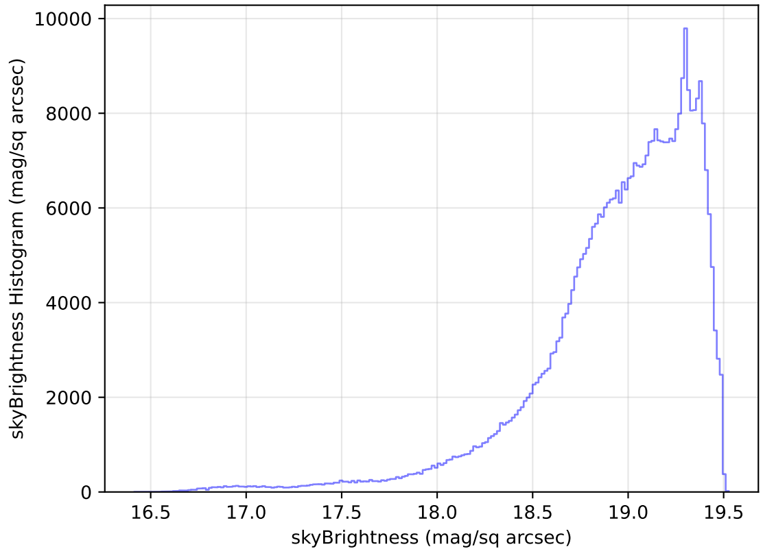
internal_u_expt38_nscale1.5v3.4_10yrs All sky z band: skyBrightness Histogram
