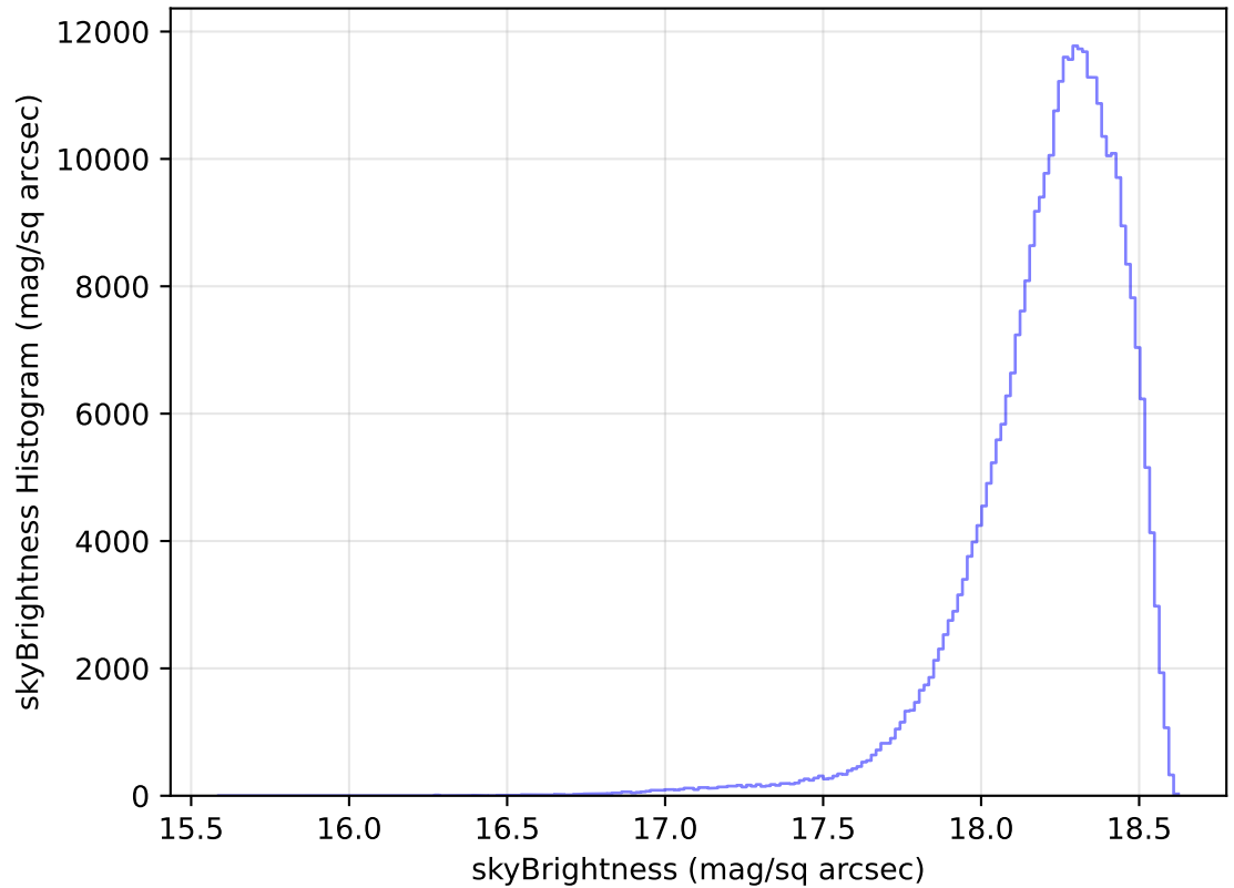
internal_u_expt38_nscale1.5v3.4_10yrs All sky y band: skyBrightness Histogram
