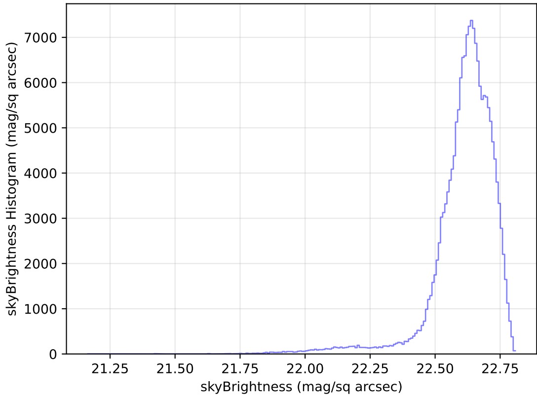
internal_u_expt38_nscale1.5v3.4_10yrs All sky u band: skyBrightness Histogram
