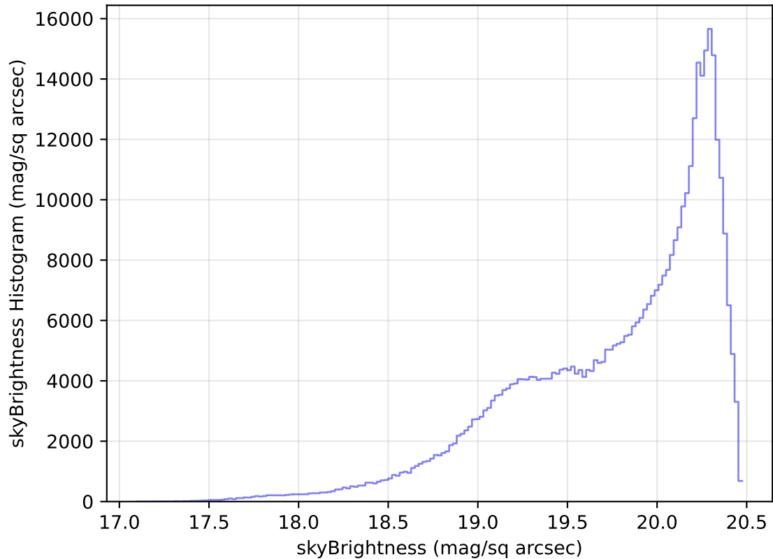
internal_u_expt38_nscale1.5v3.4_10yrs All sky i band: skyBrightness Histogram
