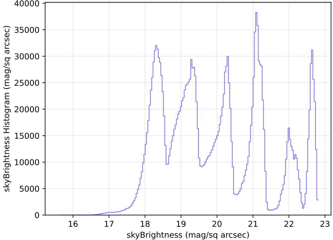
internal_u_expt38_nscale1.5v3.4_10yrs All sky all bands: skyBrightness Histogram
