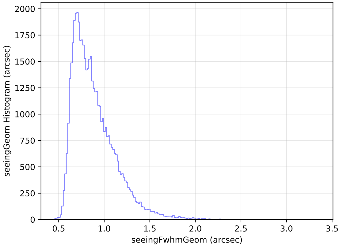
internal_u_expt38_nscale1.5v3.4_10yrs Yr 1 r band: seeingGeom Histogram
