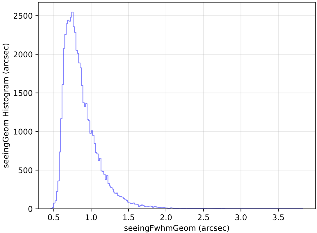
internal_u_expt38_nscale1.5v3.4_10yrs Yr 1 i band: seeingGeom Histogram
