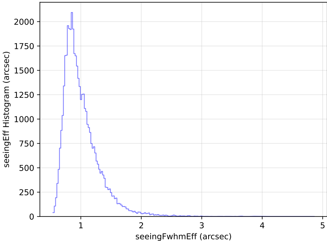
internal_u_expt38_nscale1.5v3.4_10yrs Yr 1 z band: seeingEff Histogram
