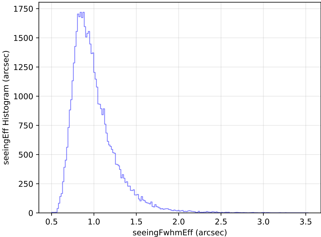
internal_u_expt38_nscale1.5v3.4_10yrs Yr 1 y band: seeingEff Histogram
