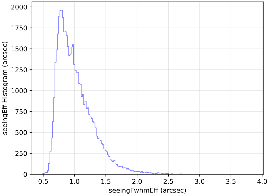
internal_u_expt38_nscale1.5v3.4_10yrs Yr 1 r band: seeingEff Histogram
