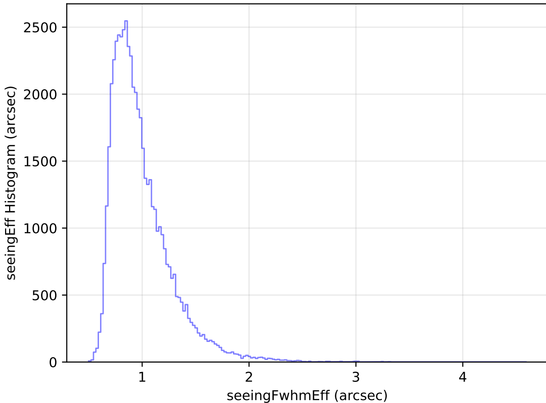
internal_u_expt38_nscale1.5v3.4_10yrs Yr 1 i band: seeingEff Histogram
