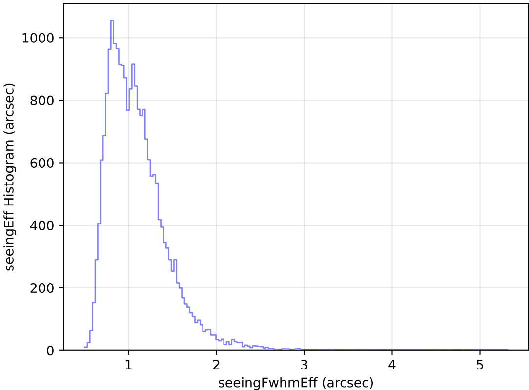
internal_u_expt38_nscale1.5v3.4_10yrs Yr 1 g band: seeingEff Histogram
