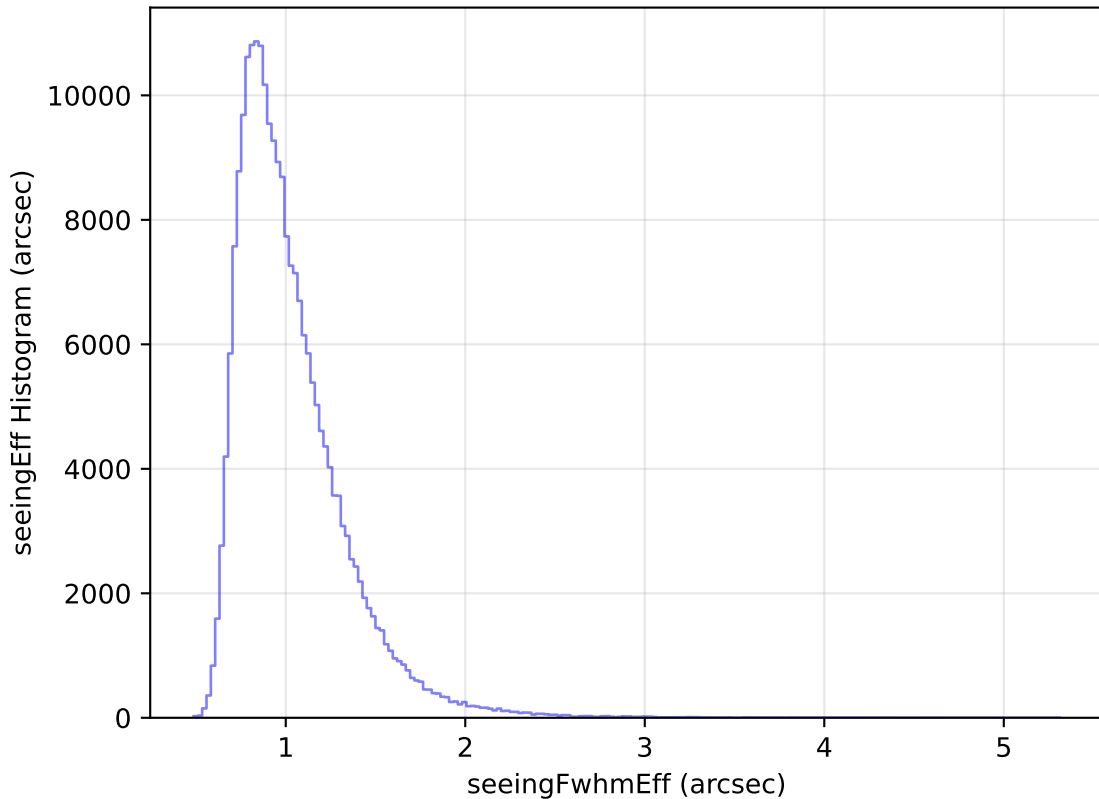
internal_u_expt38_nscale1.5v3.4_10yrs Yr 1 all bands: seeingEff Histogram
