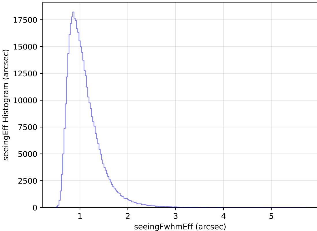
internal_u_expt38_nscale1.5v3.4_10yrs WFD z band: seeingEff Histogram
