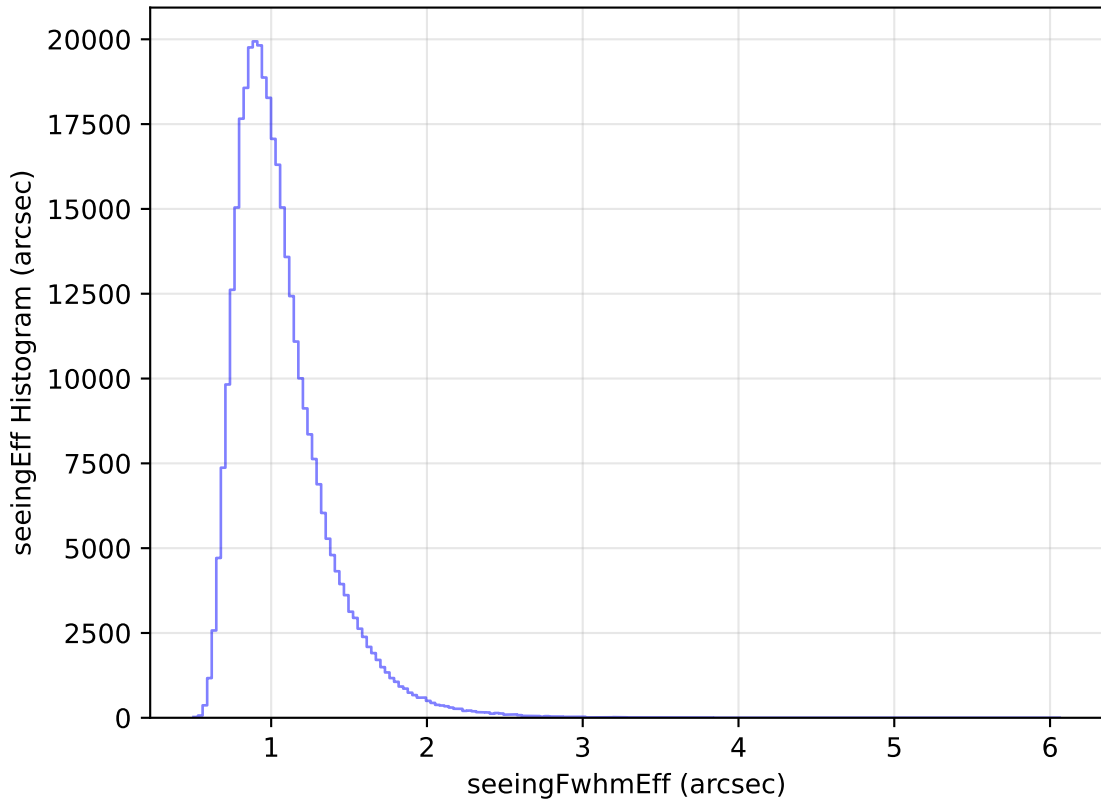
internal_u_expt38_nscale1.5v3.4_10yrs WFD y band: seeingEff Histogram
