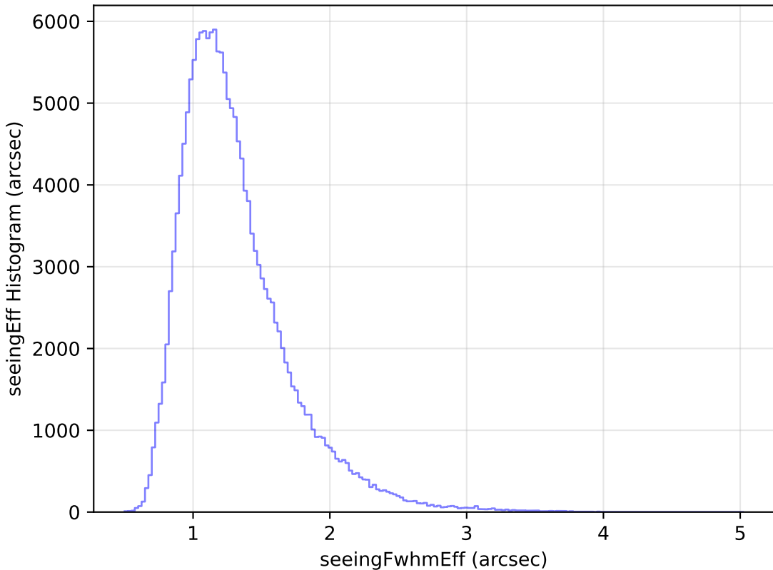
internal_u_expt38_nscale1.5v3.4_10yrs WFD u band: seeingEff Histogram
