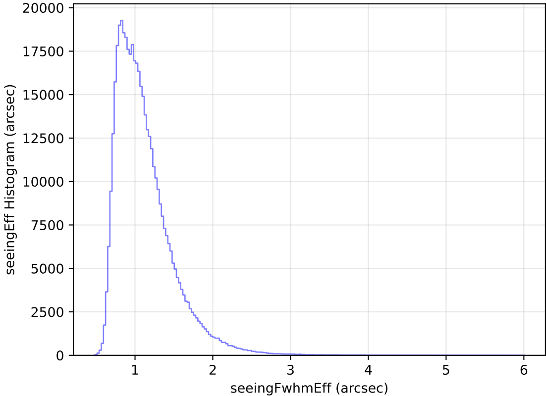
internal_u_expt38_nscale1.5v3.4_10yrs WFD r band: seeingEff Histogram
